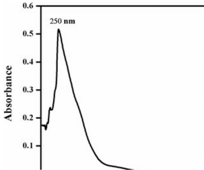
Fig. 1 – 1 UV absorption spectrum of chitosan nanoparticles (a way to absorb energy)
